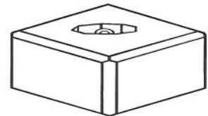
Half Flat Half Height 750mm x 750mm x 375mm 475Kg
